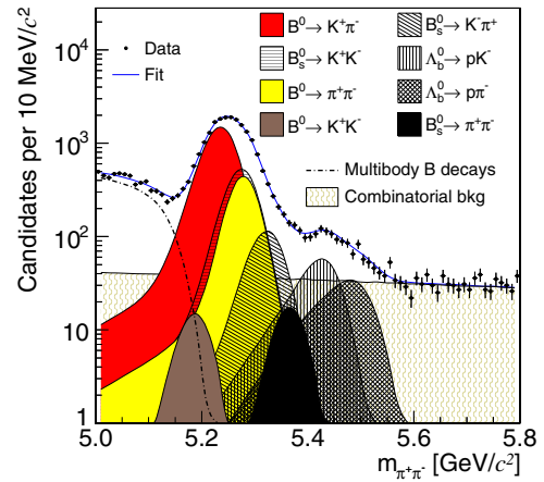
FIG. 1 (color online). Mass distribution of reconstructed candidates, where the charged pion mass is assigned to both tracks. The sum of the fitted distributions and the individual components ( C -conjugate decay modes are also implied) of the signal and background is overlaid on the data distribution.
