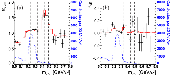
FIG. 2 (color online). Distribution of the average value of \kappa_{\text{sum}} (a) and \kappa_{\text{dif}} (b) as a function of m_{\pi^+\pi^-} . The fit function is overlaid. For reference, the distribution of m_{\pi^+\pi^-} is shown by the dashed lower histogram. Dashed vertical lines indicate the position, from left to right, of the following signals: B^0 \rightarrow K^+\pi^- , B_s^0 \rightarrow K^-\pi^+ , \Lambda_b^0 \rightarrow pK^- , \Lambda_b^0 \rightarrow p\pi^- .
