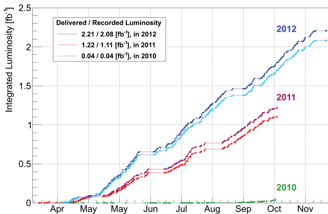
Fig. 4. Integrated luminosity in LHCb during the three years of LHC Run I. The figure shows the curves for the delivered (dark coloured lines) and recorded (light coloured lines) integrated luminosities.
