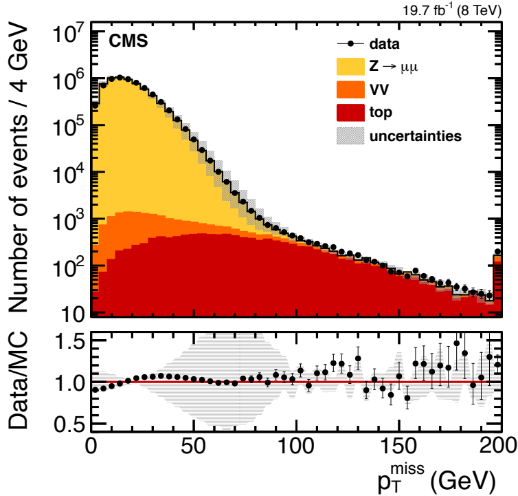
Figure 26. Spectrum of PF p_T^{\text{miss}} in a Z \rightarrow \mu\mu data set [47]. The observed data are compared to simulated Z \rightarrow \mu\mu , diboson ( VV ), and t\bar{t} plus single top quark events. The lower panel shows the ratio of data to simulation, with the uncertainty bars of the points including the statistical uncertainties of both observed and simulated events and the grey uncertainty band displaying the systematic uncertainty in the simulation. The last bin contains the overflow.
