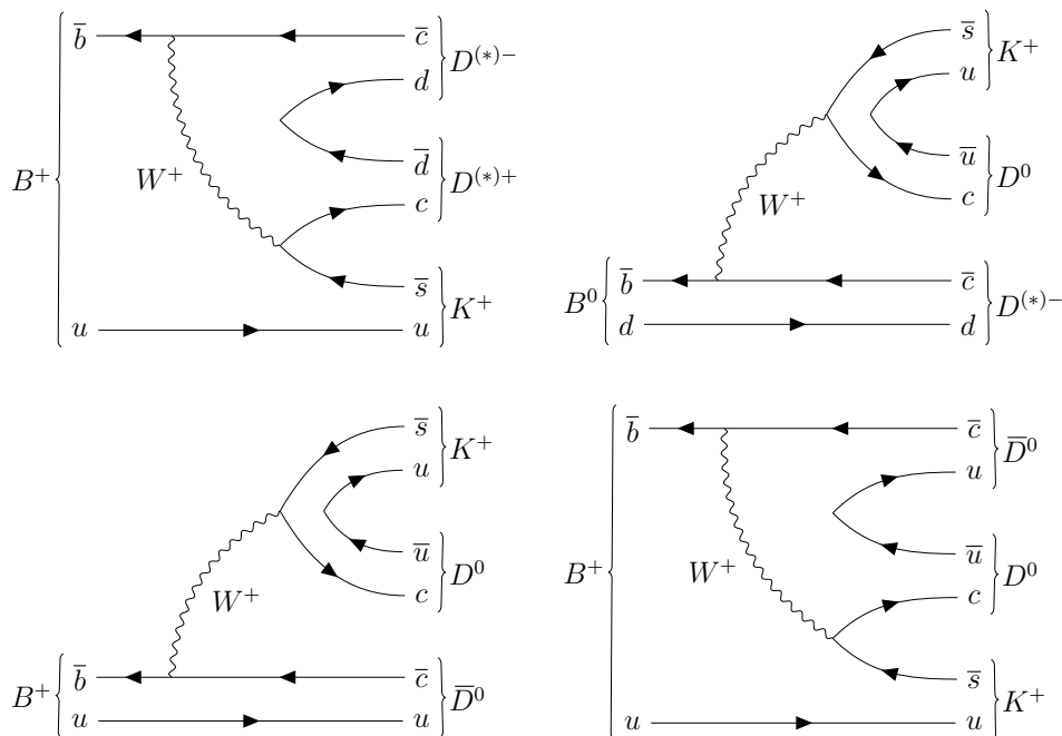
Figure 1. Top left: internal W -emission diagram for the decays B^+ \rightarrow D^{*-}D^+K^+ and B^+ \rightarrow D^{*+}D^-K^+ . Top right: external W -emission diagram for the decays B^0 \rightarrow D^{*-}D^0K^+ and B^0 \rightarrow D^-D^0K^+ . Bottom row: (left) external and (right) internal W -emission diagrams contributing to the B^+ \rightarrow \bar{D}^0D^0K^+ decay.
