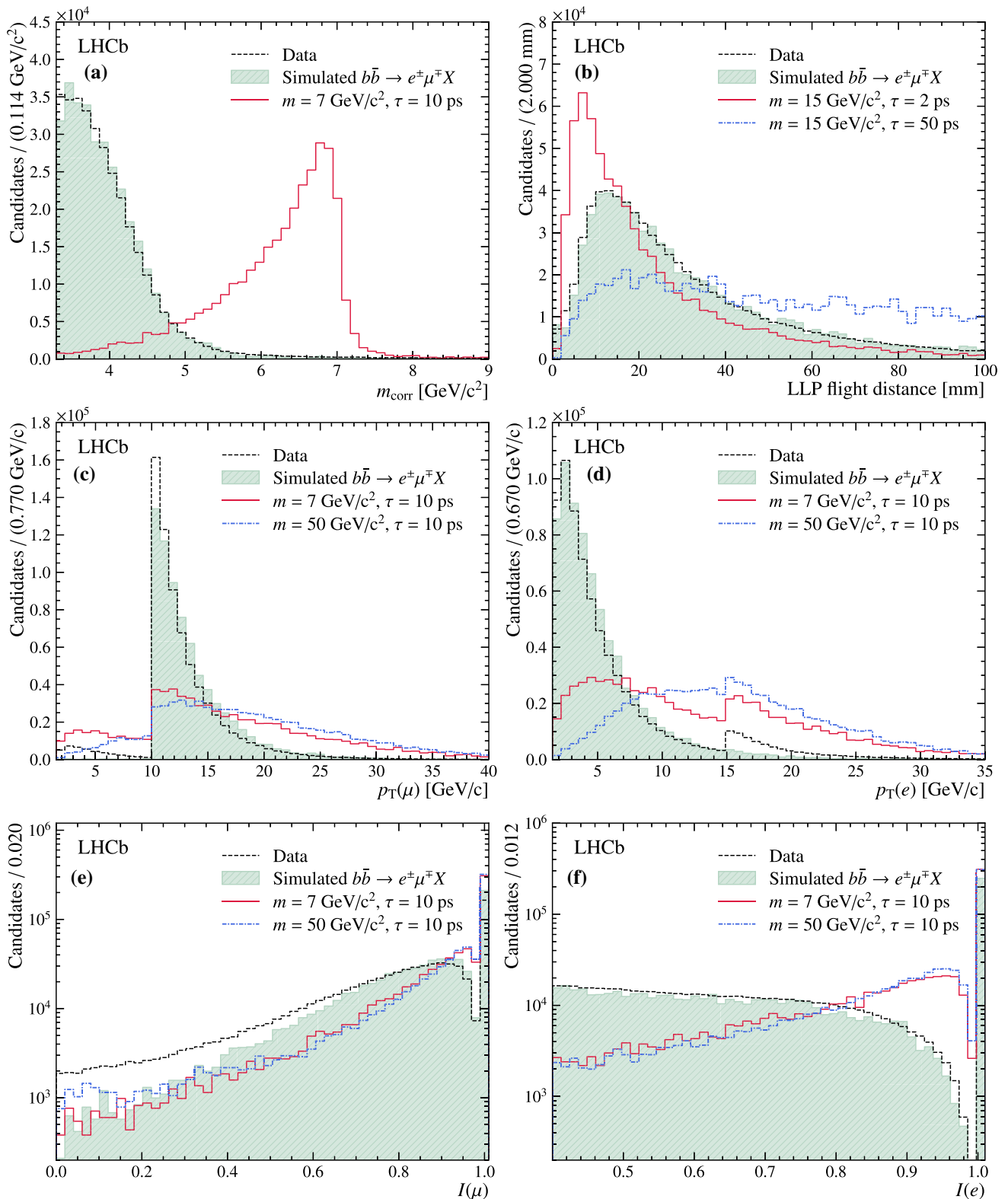
Fig. 2 Distributions in data (dashed black histogram) compared to simulated b\bar{b} \rightarrow e^\pm \mu^\mp X (green filled histogram), showing, a m_{corr} , b the LLP flight distance, c the transverse momentum of the muon, d the transverse momentum of the electron, e the isolation of the muon, and f the isolation of the electron. LLP signal distributions are also shown (coloured histograms) for different m_{LLP} and \tau_{LLP} values, where the
