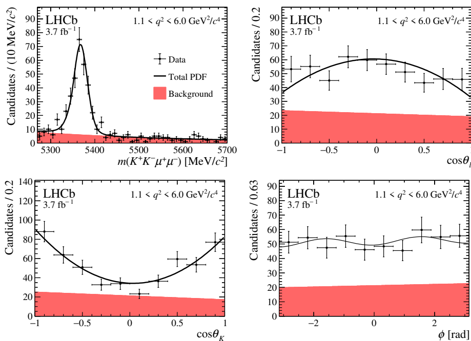
Figure 29. Mass and angular distributions of B_s^0 \rightarrow \phi\mu^+\mu^- candidates in the region 1.1 < q^2 < 6.0 \text{ GeV}^2/c^4 for data taken in 2017–2018. The data are overlaid with the projections of the fitted PDF.
