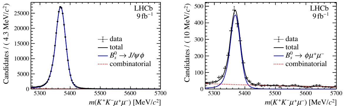
FIG. 1. Reconstructed invariant mass of the K^+K^-\mu^+\mu^- system for (left) the B_s^0 \rightarrow J/\psi\phi normalization mode and (right) the B_s^0 \rightarrow \phi\mu^+\mu^- signal candidates, integrated over q^2 and overlaid with the fit projections.
