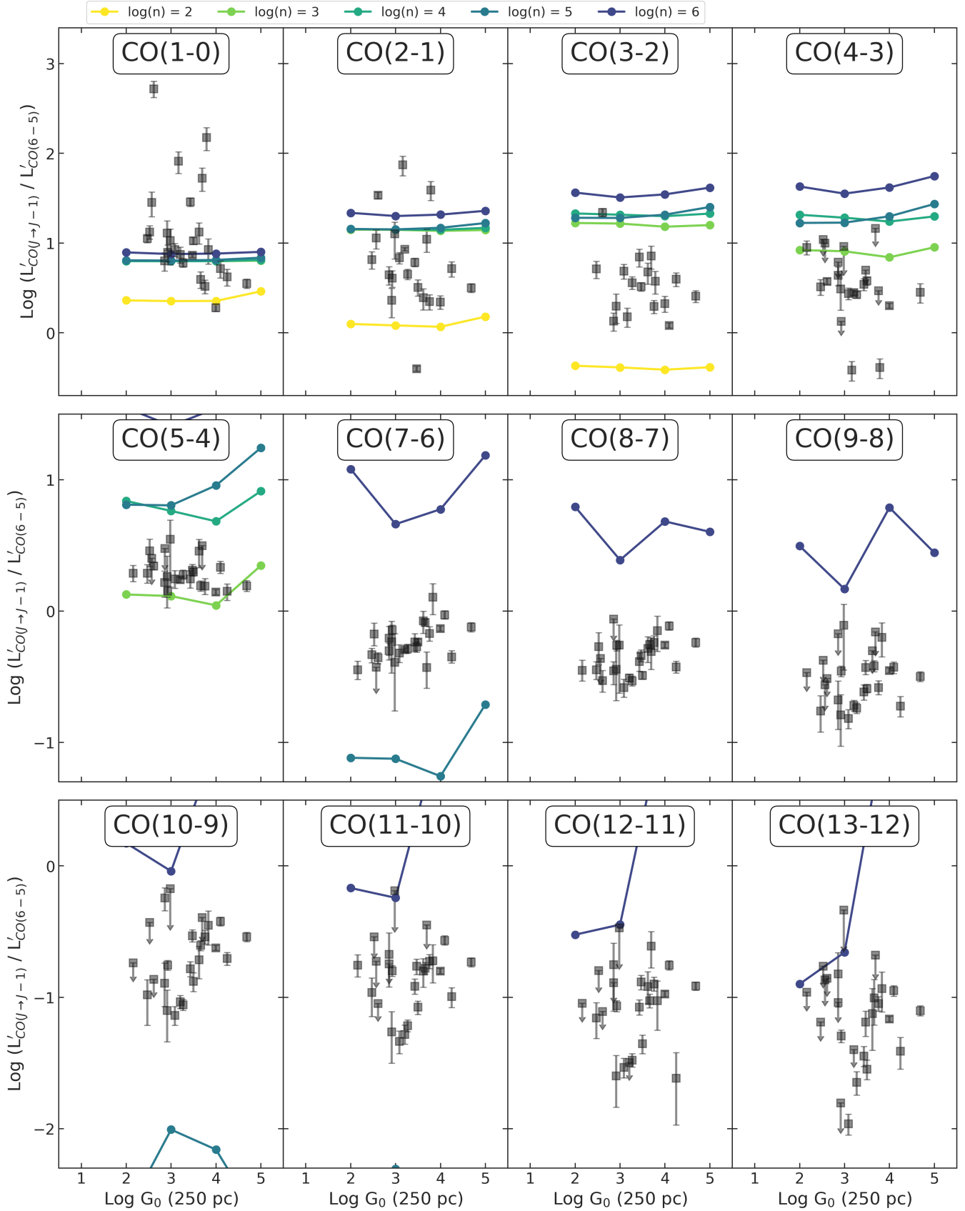
Figure A6. CO line ratios, with respect to the CO(6–5) line, vs. G_0 . The x-axis is the Habing field G_0 (for r = 250 pc). The y-axis is the luminosity ratio L'_{\text{CO}(j \rightarrow j-1)} / L'_{\text{CO}(6-5)} to the CO(6–5) line. Data points and lines are described in Figure A5.
