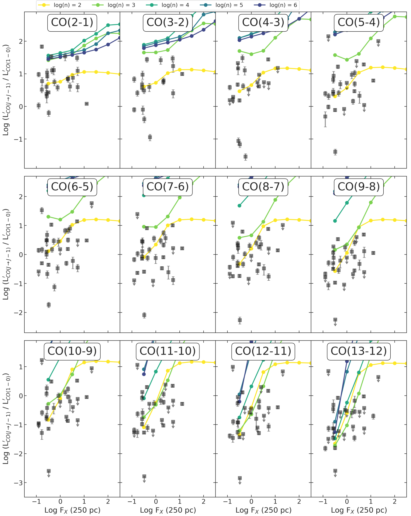
Figure A7. CO line ratios, with respect to the CO(1–0) line, vs. F_X . The x-axis is F_X (for r = 250 pc), in units of \text{erg s}^{-1} \text{cm}^{-2} . The y-axis is the luminosity ratio L'_{\text{CO}(J \rightarrow J-1)} / L'_{\text{CO}(1 \rightarrow 0)} to the nuclear ( r = 250 pc) fraction of CO(1–0). Data points and lines are described in Figure A5.
