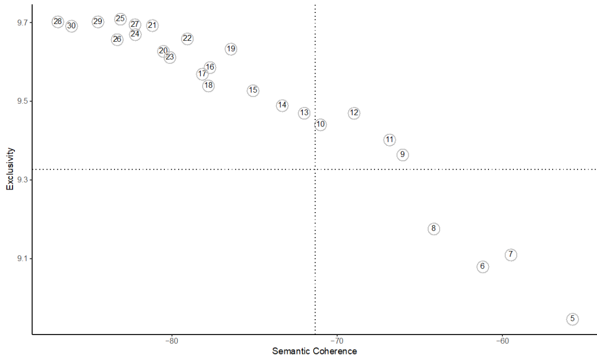
Figure 1: Exclusivity and Semantic Coherence of Topic Models in the Range between 5 and 30 Topics
