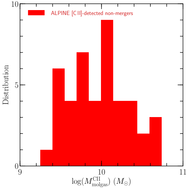
Fig. 1. Distribution of molecular gas masses of the 44 ALPINE [C II]-detected nonmerger galaxies at z = 4.4\text{--}5.9 . The molecular gas masses were derived using the calibration of Zanella et al. (2018) between [C II] luminosity and molecular gas mass (Eq. (1)).
