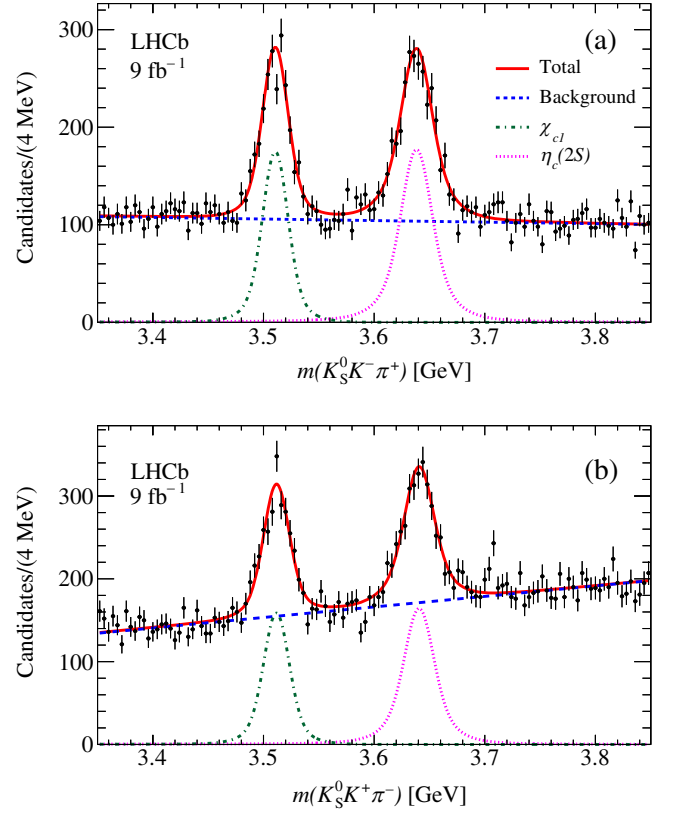
FIG. 5. Invariant K_S^0 K \pi mass distributions in the \chi_{c1} - \eta_c(2S) mass region for (a) B^+ \rightarrow K_S^0 K^- \pi^+ and (b) B^+ \rightarrow K_S^0 K^+ \pi^- candidates. The results of the fits are overlaid.
