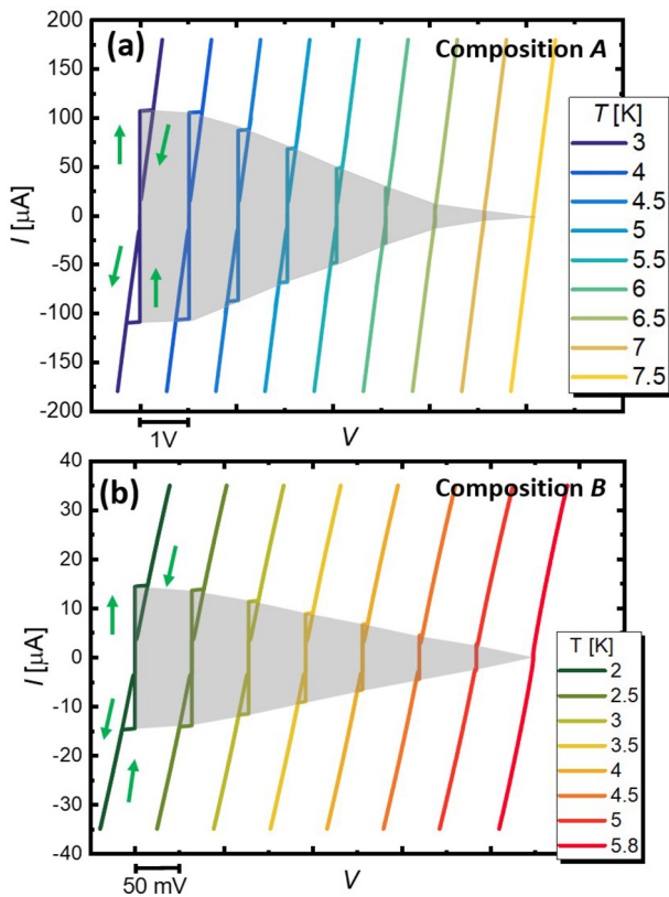
FIG. 2. [(a) and (b)]; Current vs voltage ( I - V ) characteristics for selected values of the bath temperature (in legend) for device 1A [(1B)]. The green arrows represent the current direction in the different branches of the curve. The gray areas correspond to the dissipationless region. The curves are horizontally shifted for clarity; each tick in the graph represents 1 V for panel a and 50 mV for panel (b).
