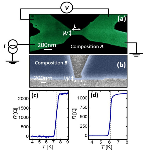
FIG. 1. (a) False color scanning electron micrograph (SEM) of one representative Dayem-bridge device with composition A. The four-wire measurement setup and the characteristic nanobridge lateral dimensions are also indicated. I indicates the current flowing through the device, while V indicates the voltage drop occurring across it. (b) False color SEM image of a representative device with composition B (the same four-wire setup was used for this device). (c) Resistance vs temperature curve ( R vs T ) of the device shown in panel (a). (d) R vs T of the device shown in panel (b). The dashed lines indicate the critical temperatures T_c^{\text{exp}} of the shown devices.
