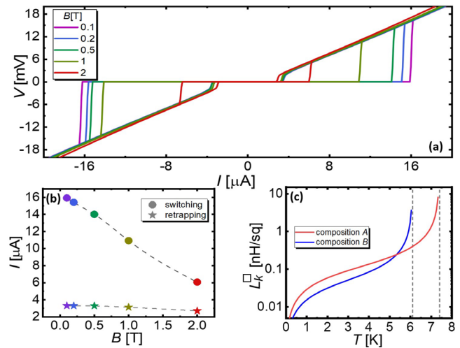
FIG. 4. (a) I - V characteristics as a function of perpendicular-to-plane magnetic field B applied to a representative device with composition B. (b): Switching and retrapping currents of the curves in (a) as a function of B . Dashed lines are guides to the eye. (c): Kinetic inductance per square L_K^{\square} as a function of temperature T for samples 1A and 1B. Dashed lines indicate the asymptotes of L_K^{\square} due to \Delta(T) approaching 0 at T = T_c . All the measurements shown in panels (a) and (b) were taken at T_{bath} = 2 K.
