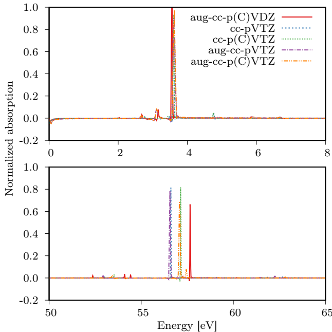
FIG. 4. Normalized aug-cc-p(C)VDZ, cc-pVTZ, cc-p(C)VTZ, aug-cc-pVTZ and aug-cc-p(C)VTZ LiH pump-probe absorption, S'(\omega) , as a function of energy. Time-dependent dipole moments are calculated using TDCCSD, and integrated with RK4 with 0.005 a.u. time steps.
