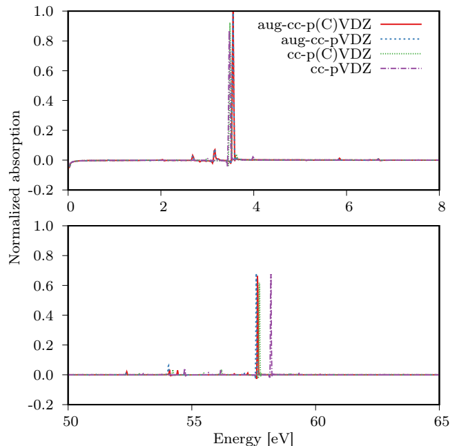
FIG. 3. Normalized aug-cc-p(C)VDZ, aug-cc-pVDZ, cc-p(C)VDZ and cc-pVDZ LiH pump and probe absorption, S'(\omega) , as a function of energy. Time-dependent dipole moments are calculated using TDCCSD, and integrated with RK4 with 0.005 a.u. time steps.
